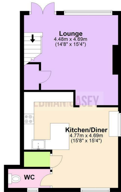
Ground Floor Approx. 41.0 sq. metres (441.3 sq. feet)
